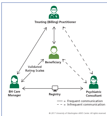
Figure 1: Illustration of a CoCM model
